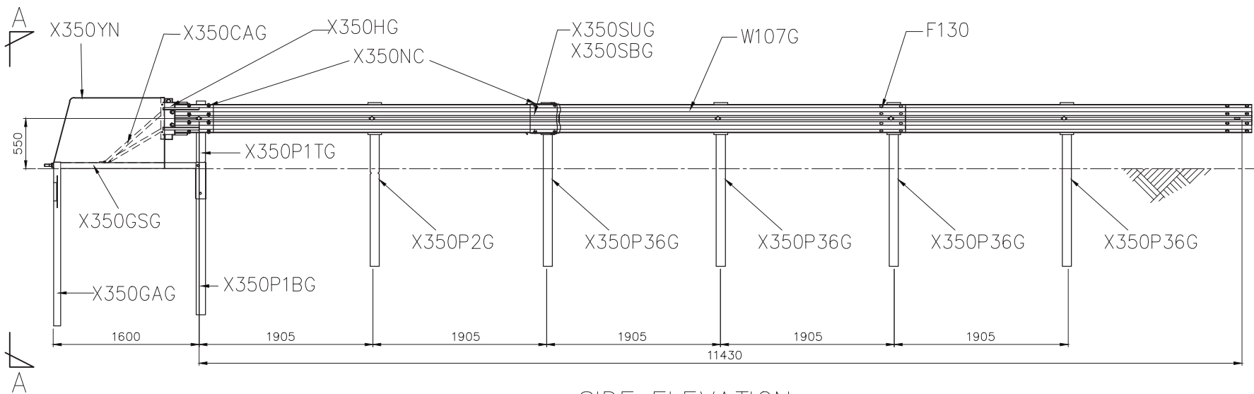
SIDE ELEVATION
