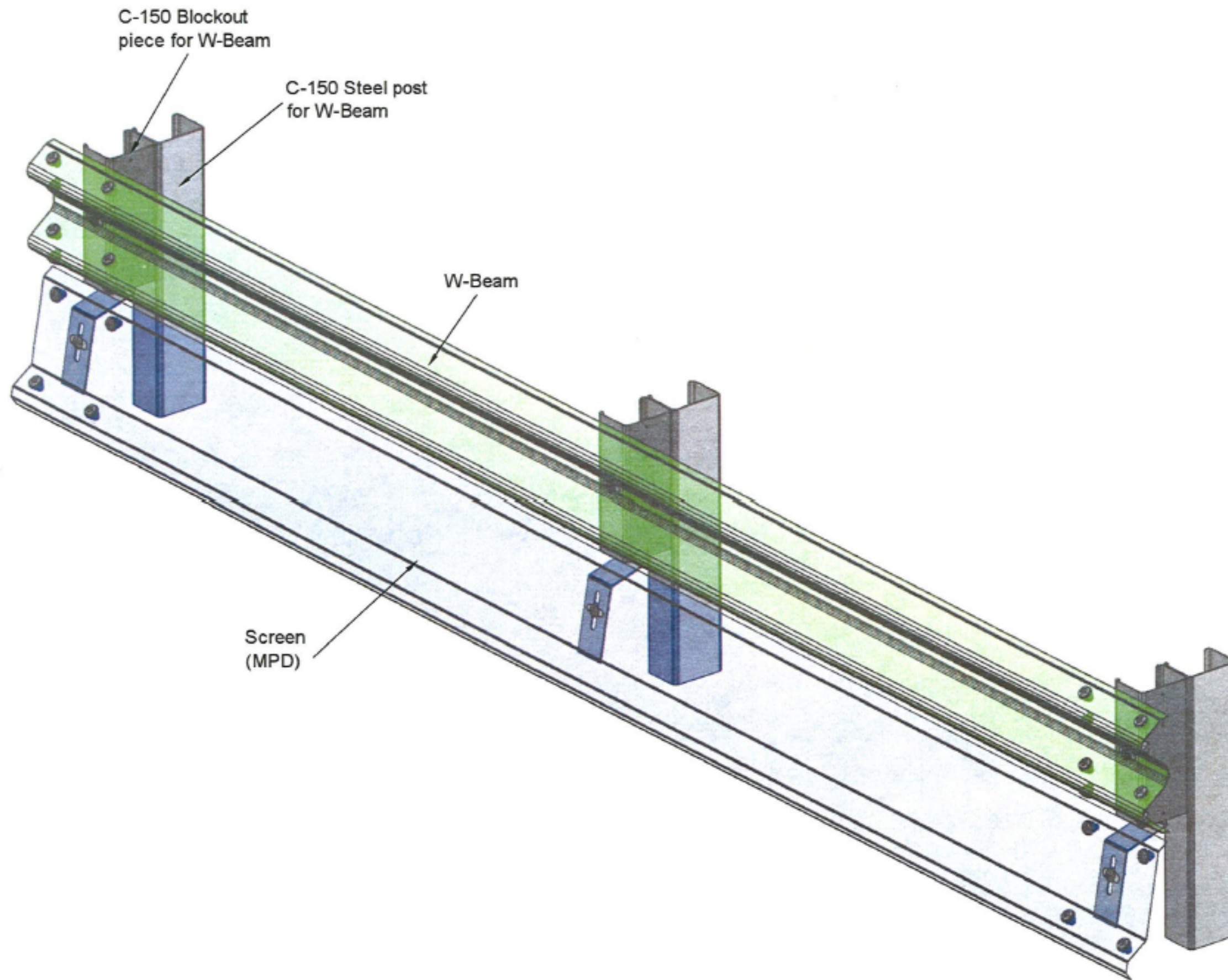
AUSTRALIAN / NEW ZEALAND STANDARD (AASHTO G4 W-BEAM) STEEL GUARDRAIL WITH MOTORCYCLIST PROTECTION DEVICE POST C-150 WITH SPACER C-150
