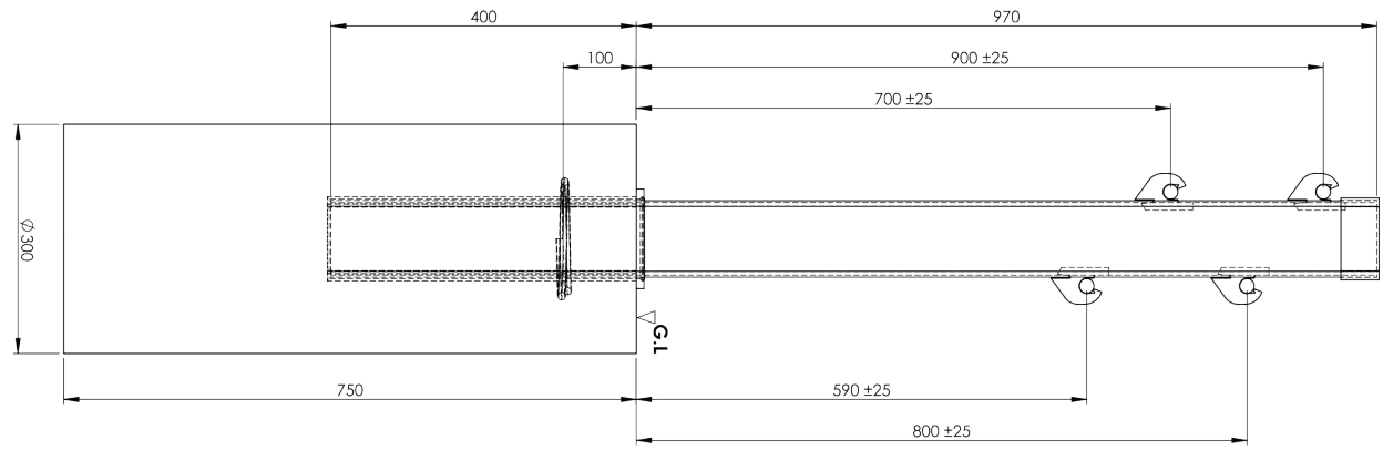
ELEVATION VIEW SCALE 1:6
