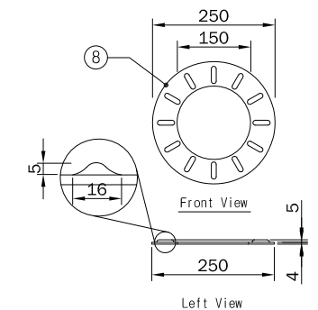
Stopper Board(9T)
