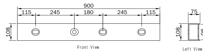
Sleeve Detail View
