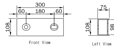
Sleeve Detail View
