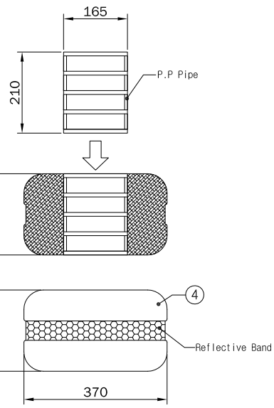
Shock Absorbing Roller Detail View
