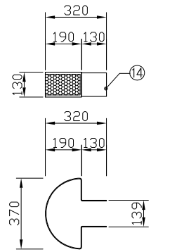
Round Rail Detail View
