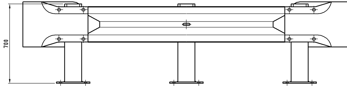
FRONT VIEW
